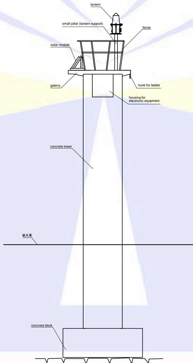
CONCRETE TOWER IN THE SEA
